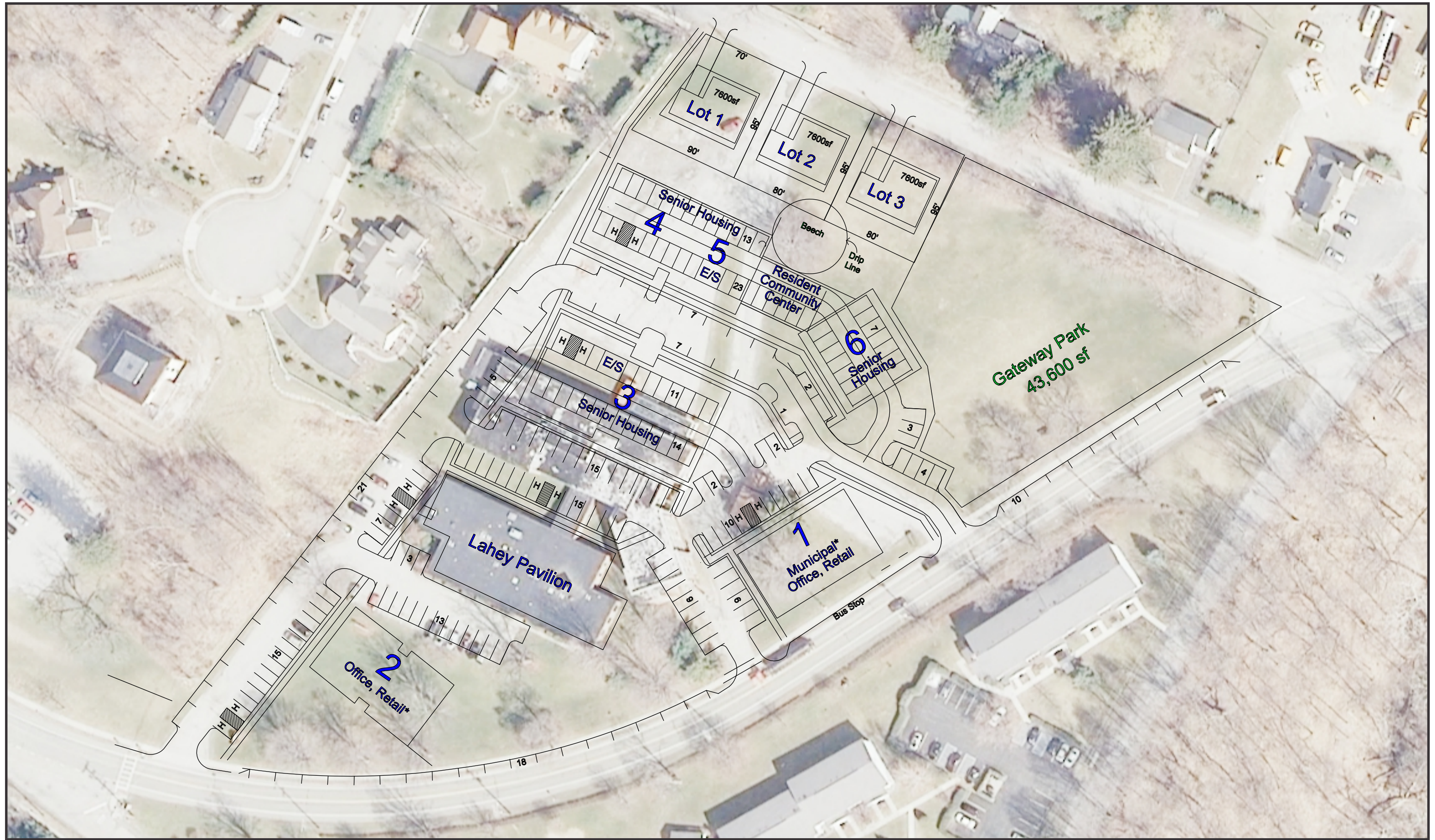
Figure 4-1: Site Plan on Aerial Photo Butterfield Village of Cold Spring, Putnam County, NY Scale: 1" = 70' Base map: NYS GIS Clearinghouse Orthoimagery, 2009
