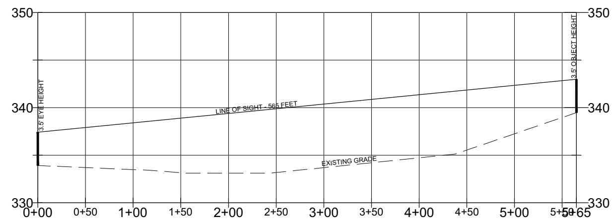
SIGHT DISTANCE PROFILE - ROAD A LOOKING LEFT VERTICAL SCALE: 1" = 10' HORIZONTAL SCALE: 1" = 100'
