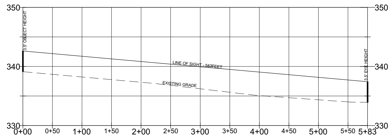
SIGHT DISTANCE PROFILE - ROAD A LOOKING RIGHT VERTICAL SCALE: 1" = 10' HORIZONTAL SCALE: 1" = 100'
