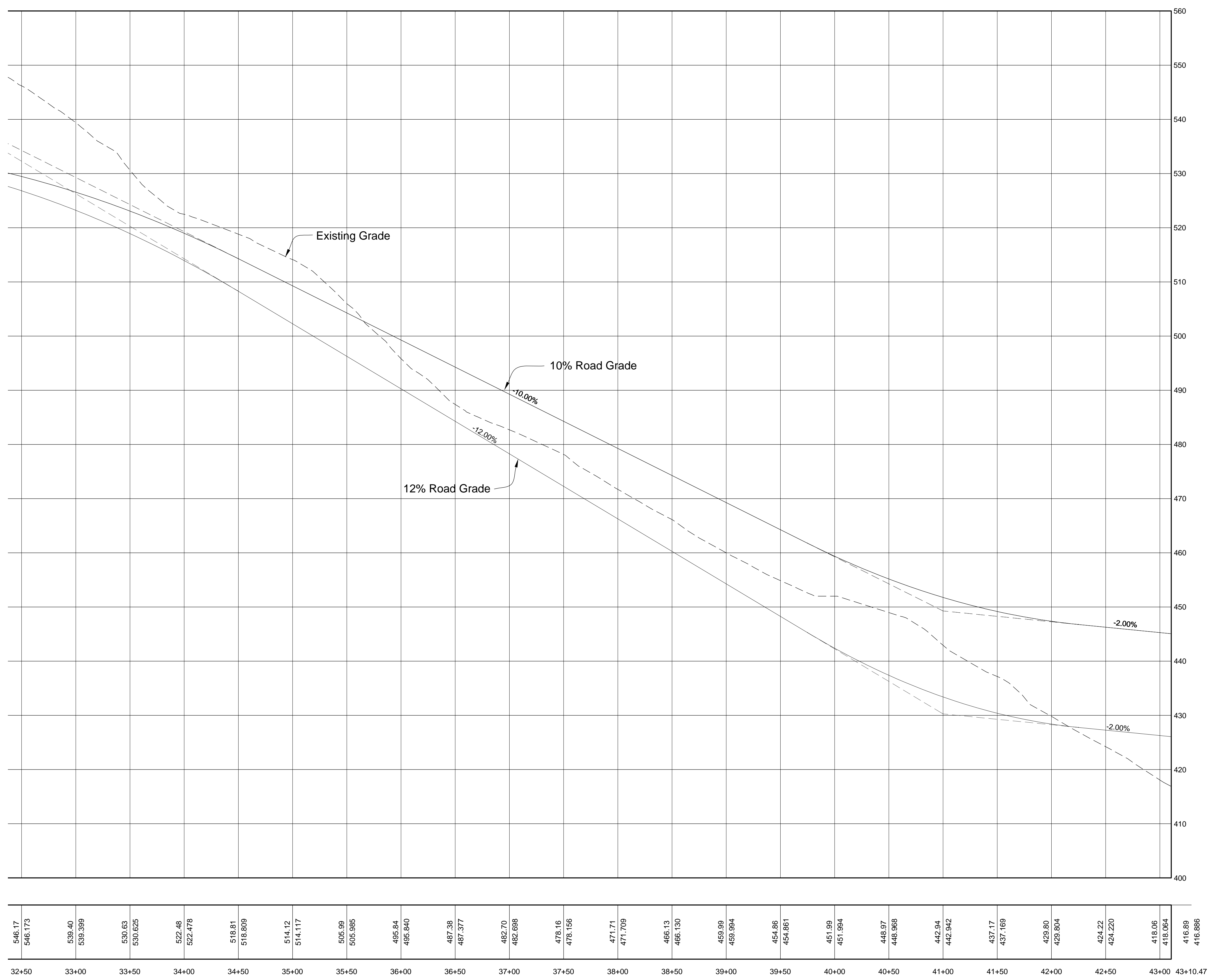
Road A Grade Profile Comparison Horizontal Scale 1"=50' Vertical Scale 1"=10'
