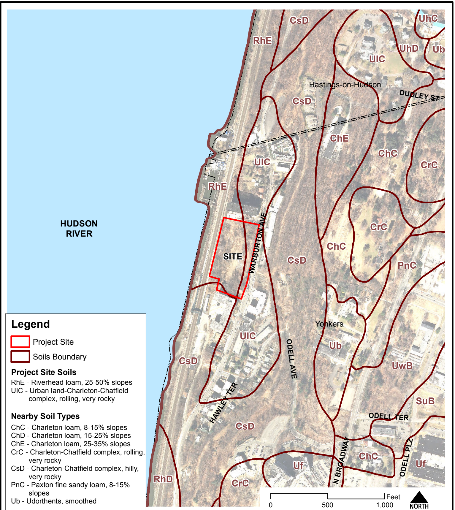
Figure 3.1-2: Soils Map River Club City of Yonkers, Westchester County, NY Source: Westchester County GIS Data, 4/7/12 Scale: As shown
