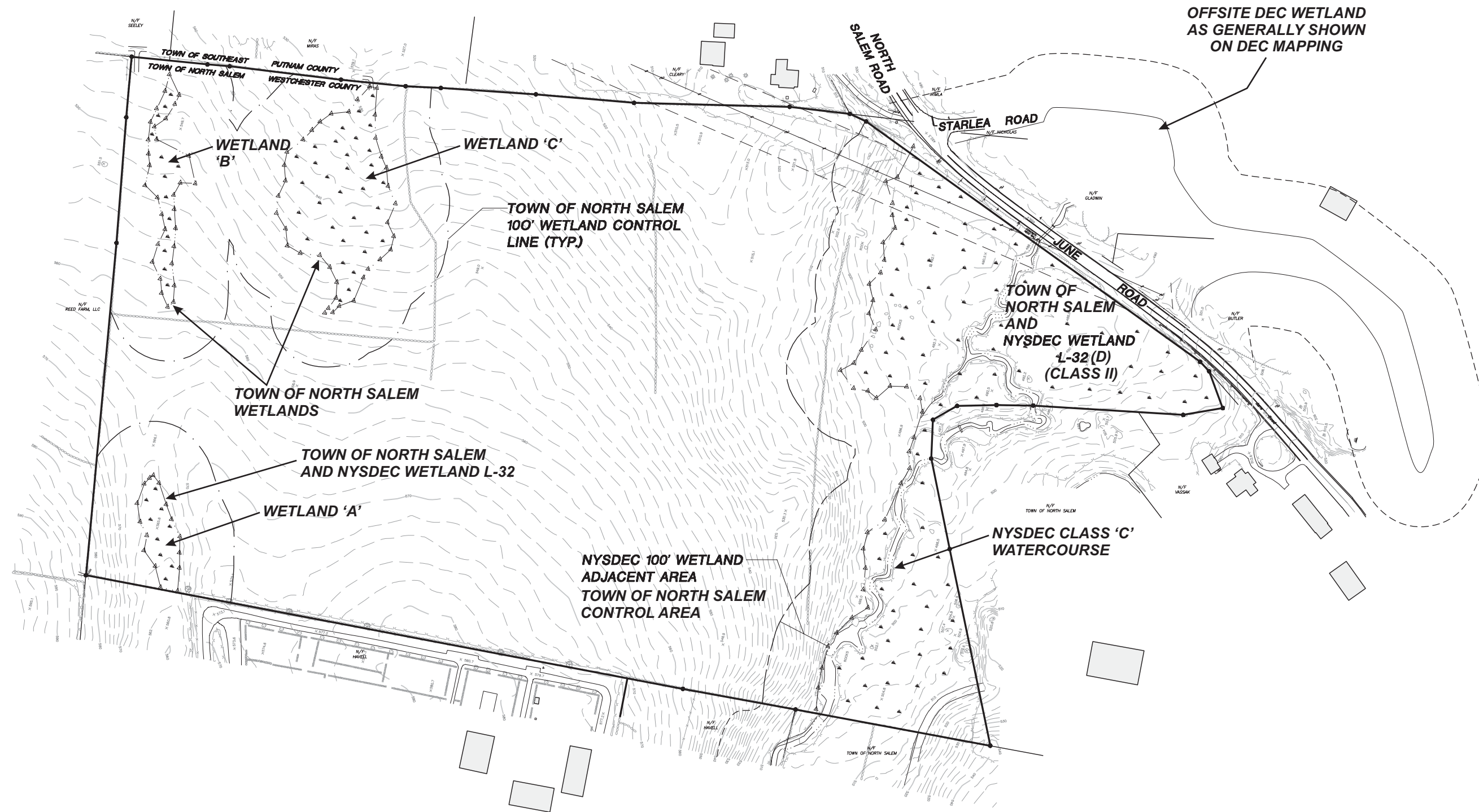
Figure 6-5: Existing Conditions Map Salem Hunt Town of North Salem, Westchester, New York Base Map: Insite Engineering, Surveying & Landscape Architecture, P.C. Date: December 1, 2006 Scale: 1 inch = 200 feet
