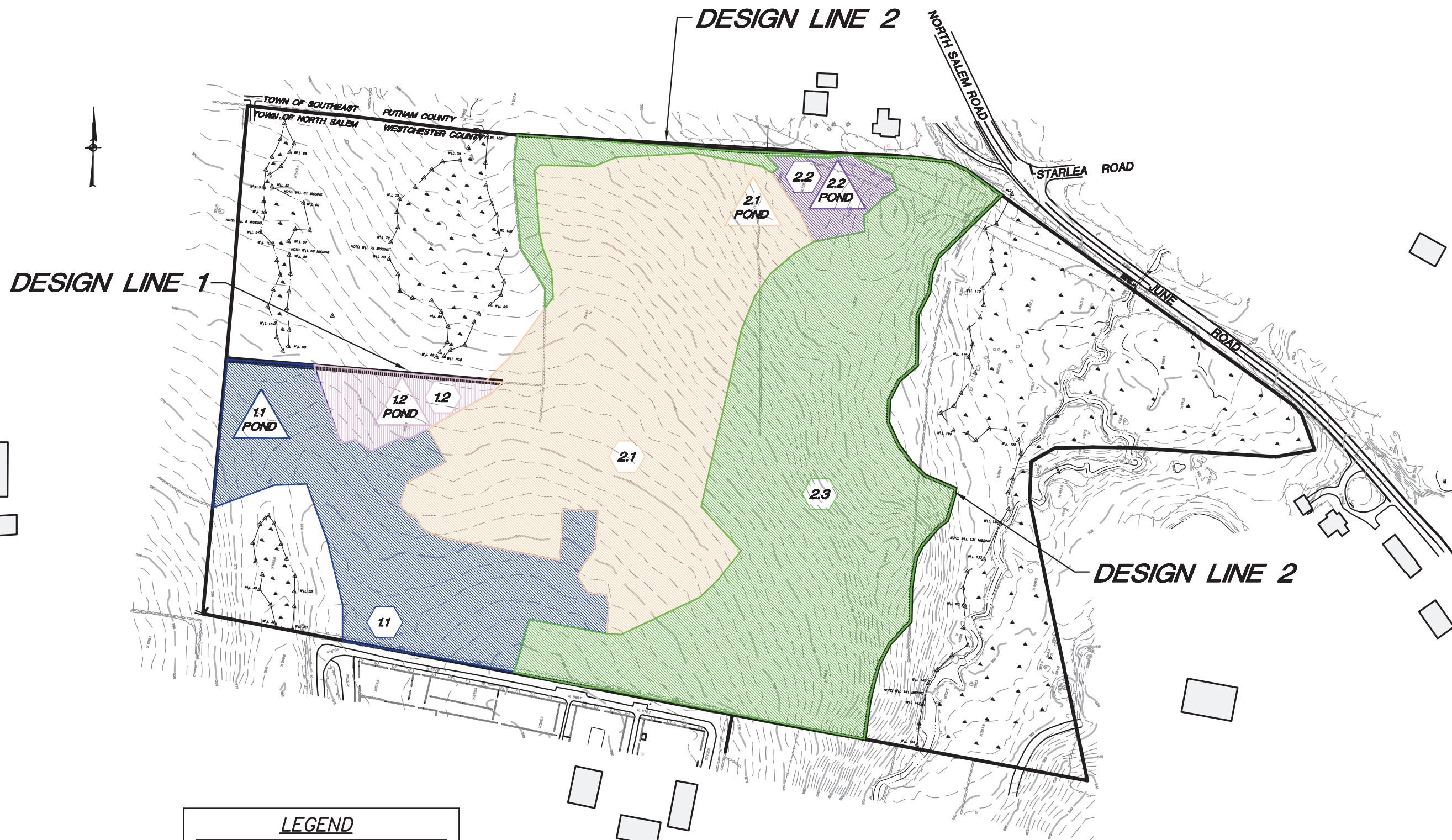
Figure 6-7: Post-Development Drainage Areas Salem Hunt Town of North Salem, Westchester, New York Base Map: Insite Engineering, Surveying & Landscape Architecture, P.C. Date: August 31, 2007 Scale: 1 inch = 200 feet
