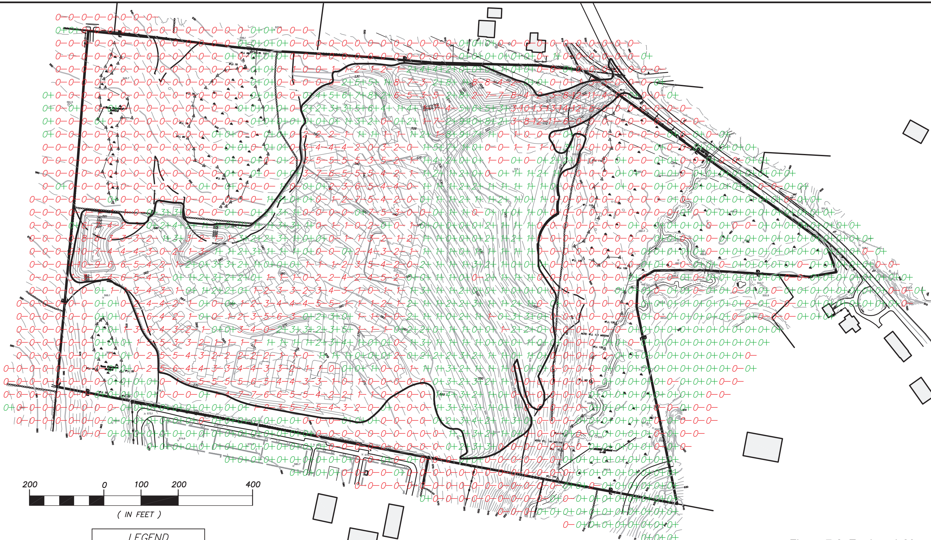
Figure 7-6: Earthwork Map Salem Hunt Town of North Salem, Westchester, New York Source: Insite Engineering, Surveying & Landscape Architecture, P.C., 8/31/07 Scale: 1" = 160'
