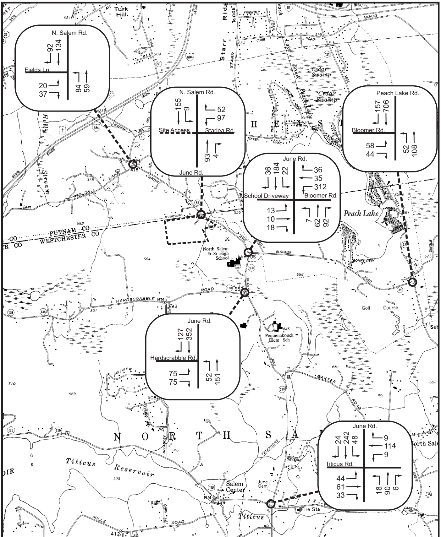
Figure 9-2: Existing AM Peak Hour Traffic Salem Hunt Town of North Salem, Westchester County, New York Base Map: U.S.D.O.T. Planimetric Map Scale: 1 inch = 2500 feet
