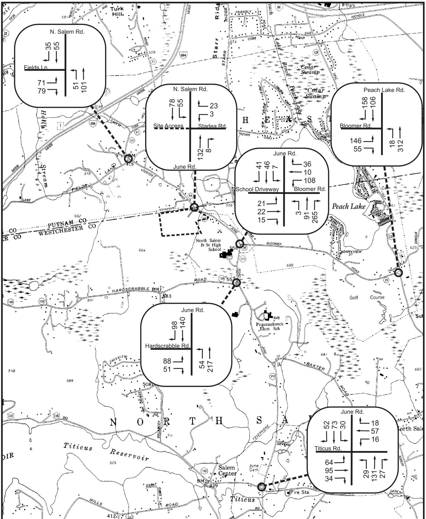
Figure 9-3: Existing PM Peak Hour Traffic Salem Hunt Town of North Salem, Westchester County, New York Base Map: U.S.D.O.T. Planimetric Map Scale: 1 inch = 2500 feet
