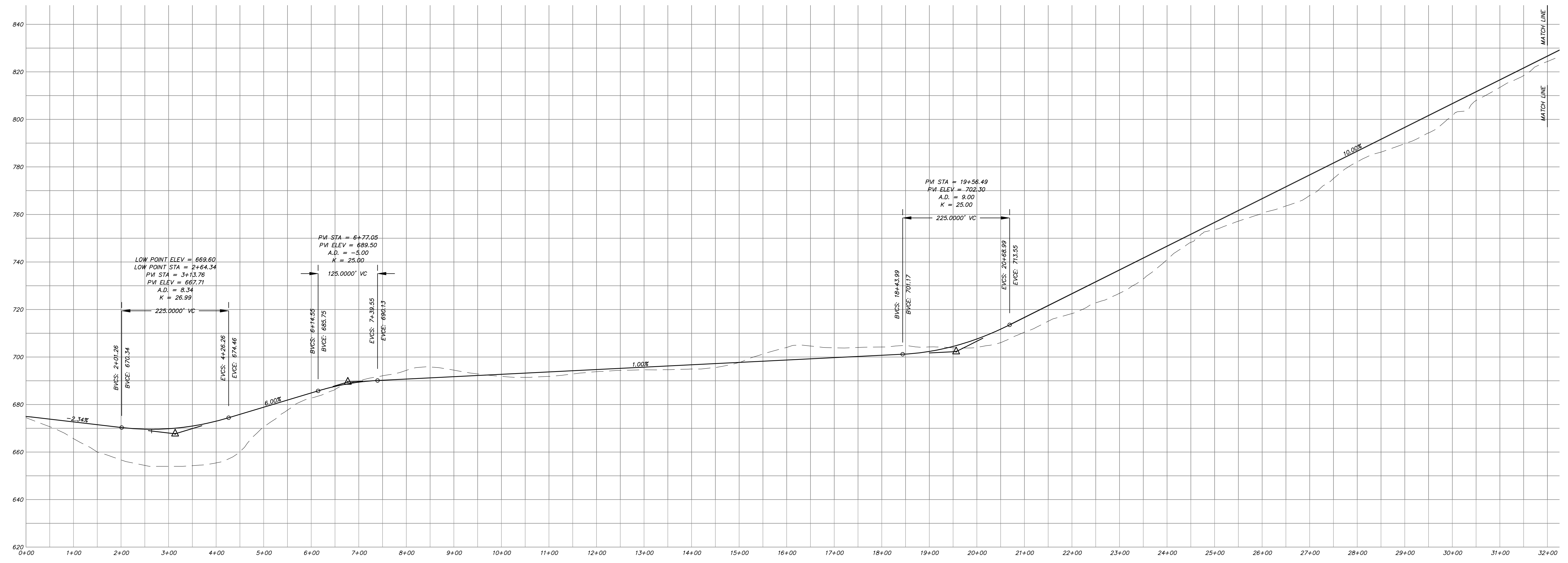
UNION HEIGHTS WEST ROAD SCALE: HORIZ. 1" = 100' VERT. 1" = 20'
