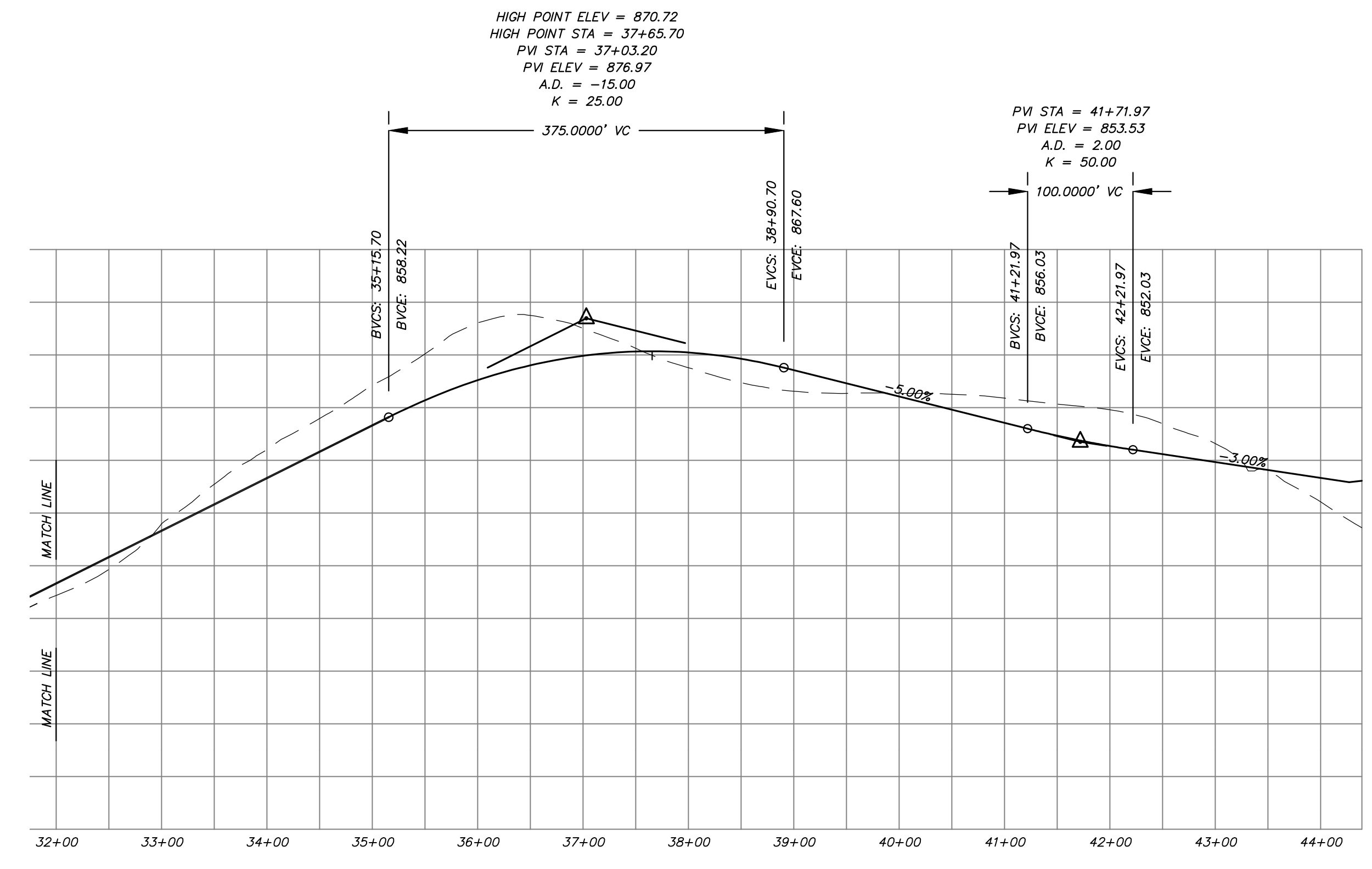
CONT. UNION HEIGHTS WEST ROAD SCALE: HORIZ. 1" = 100' VERT. 1" = 20'
