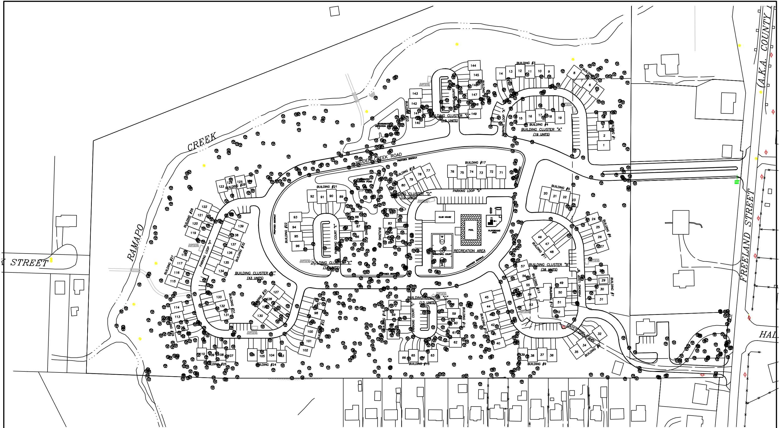
Figure 2-4: Existing Tree Coverage Hidden Creek Village of Monroe, Orange County, New York Source: Pietrzak & Pfau Engineering and Surveying, 2003 Scale: 1 inch = 175 feet
