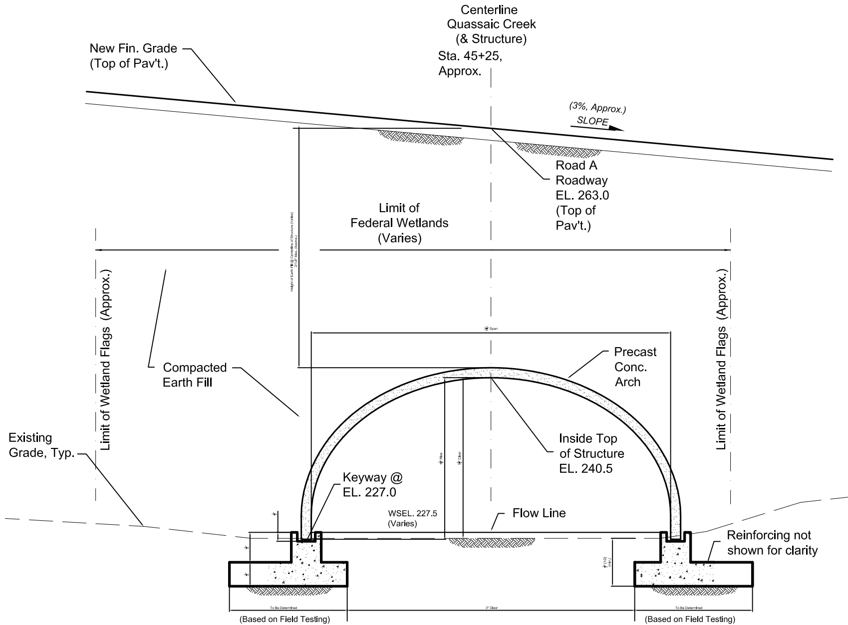
Figure 10: Quassaic Creek Crossing Proposed Access Road Over State Land Town of Newburgh, Orange County, NY Source: ACOE Wetland Permit No. NAN-2004-814 Scale: As Shown
